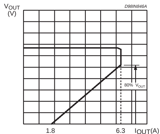
Figure 6: Output Voltage vs. Output Current. ( V_{OUT} = 1.5\text{V} )
