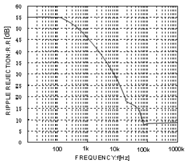
Fig.18 Ripple Rejection Characteristics ( I_{OUT}=100mA )
