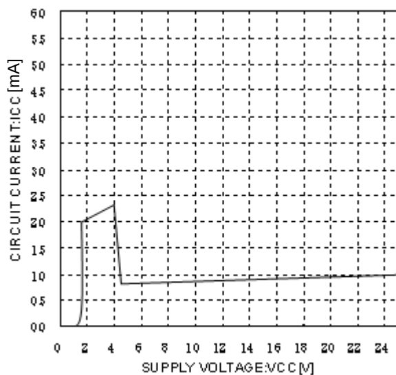
Fig.13 Circuit Current
