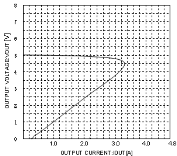
Fig.16 Load Stability
