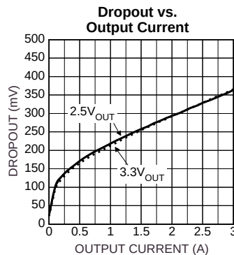
Adjustable Regulator
