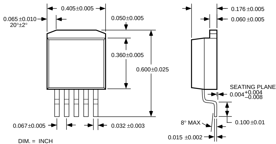
5-Lead TO-263-5 (U)
