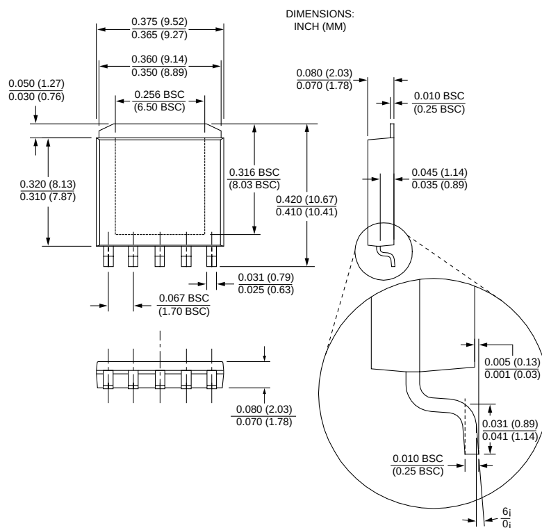
5-Lead S-PAK (R)
