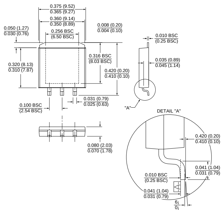
3-Lead S-PAK (R)
