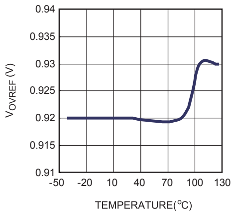
V_{OVR} vs. Temperature
