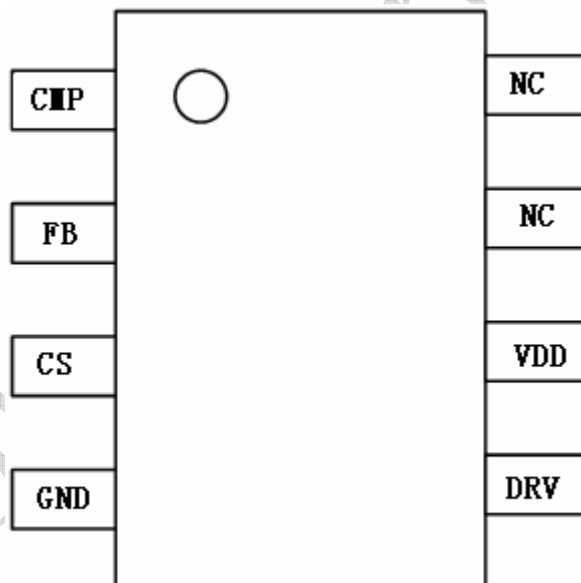
LZC811B Pin Assignmen
