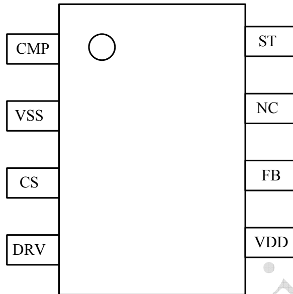
LZC811A Pin Assignmen
