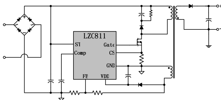
Fig 1 Application Circuit
