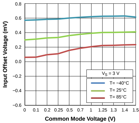
Figure 9. Input Offset Voltage vs. Common Mode Voltage at 3 V Supply
