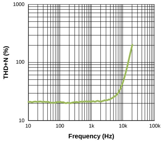
Figure 7. THD+N vs. Frequency
