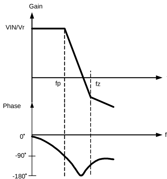
Figure 7. The Bode plot of Buck power stage
