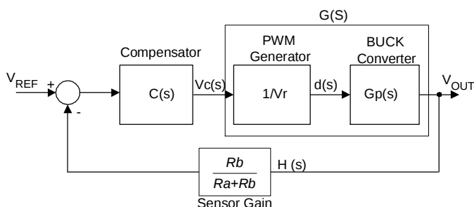
Figure 6. The control block diagram of synchronous Buck converter
