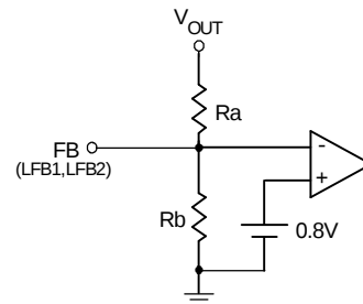
Figure 3. The connected diagram of external voltage divider and reference voltage
