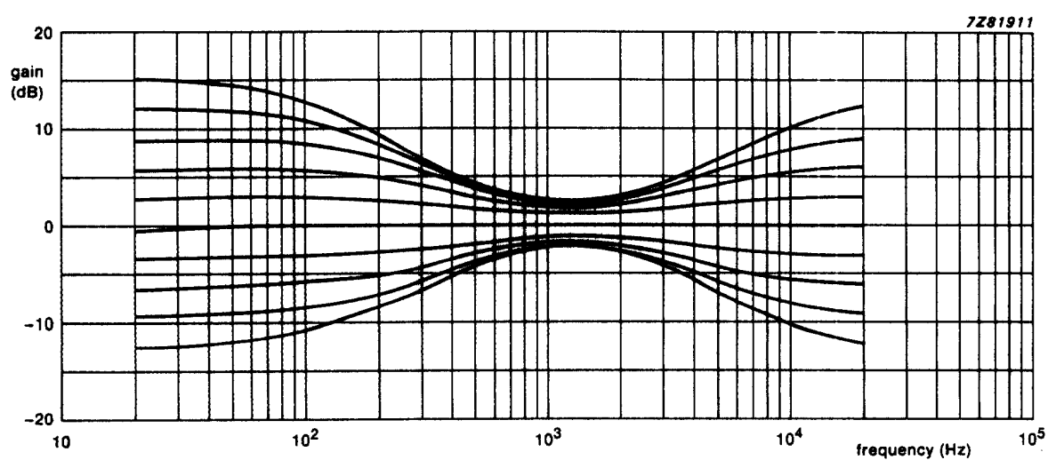
Fig.17 Frequency response of bass and treble control; bass and treble gain settings = -12 to +15 dB; gain is 0 dB; V_i = 0.1\text{ V} ; R_{S9} = 600\ \Omega ; R_L = 10\text{ k}\Omega ; V_{CC} = 12\text{ V} .
