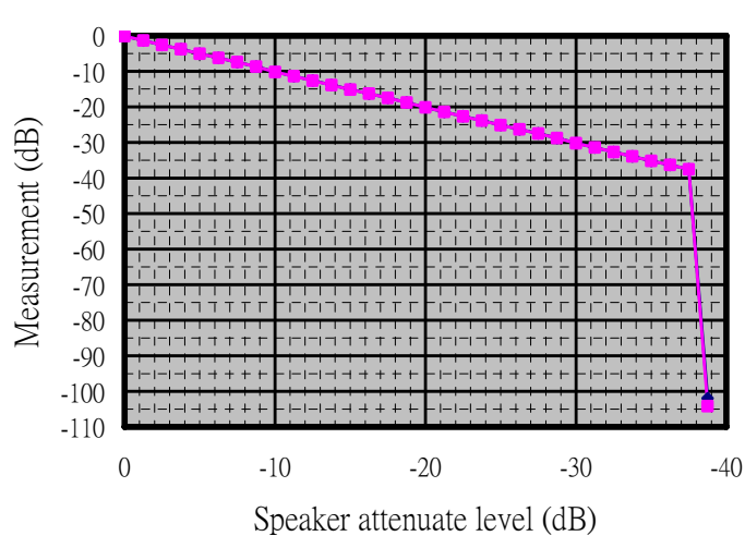
Speaker Attenuation
