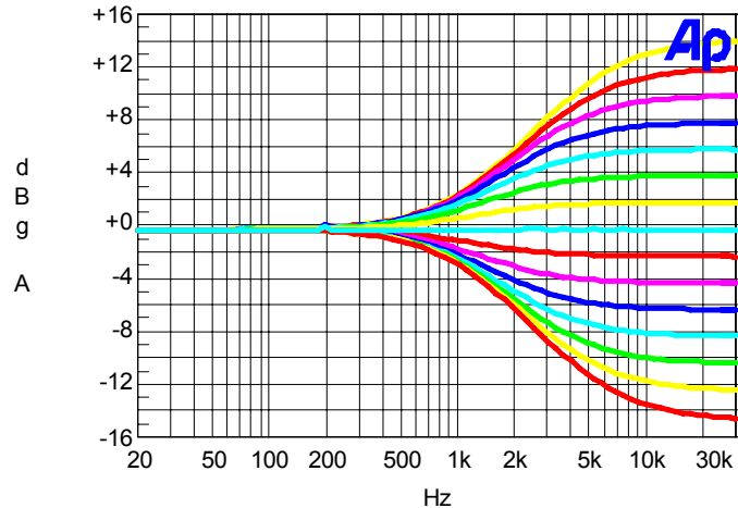
Treble Response
