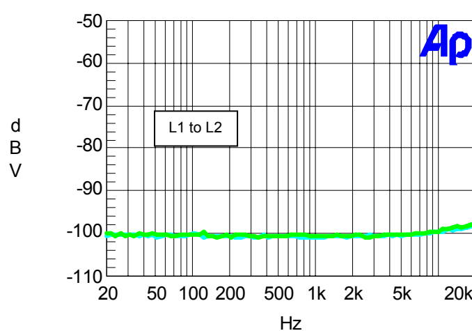
Input Selector Separation
