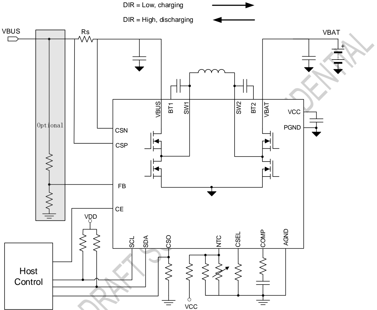
Typical application circuit 1. current sense at VBUS
