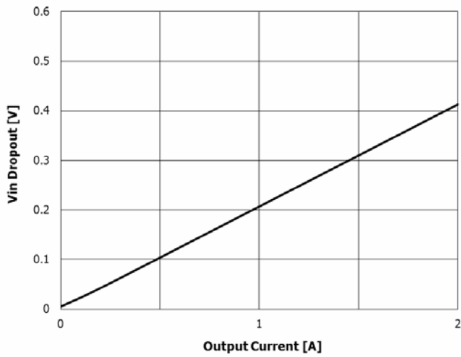
Dropout Voltage @ Vout=2.5V
