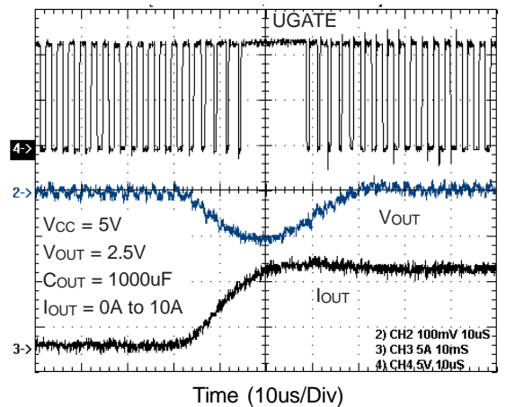
Load Transient
