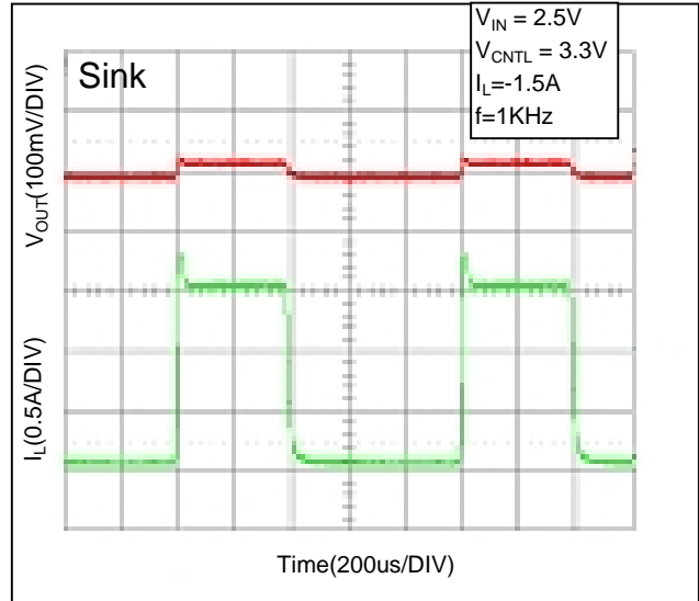
Fig 6. Transient Response
