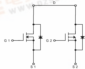
N- and P-Channel MOSFET
