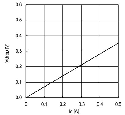
Fig.21 Minimum dropout Voltage 3 (Vcc=3.3V, Ta=25°C)
