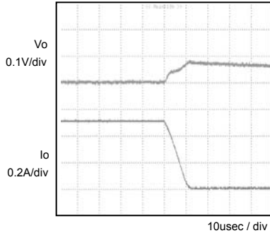
Fig.2 Transient Response ( 1.0 \rightarrow 0\text{A} ) C_o=1\mu\text{F}
