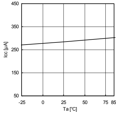
Fig.8 T_a - I_{cc}
