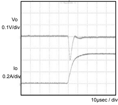
Fig.1 Transient response( 0 \rightarrow 1.0\text{A} ) C_o=1\mu\text{F}
