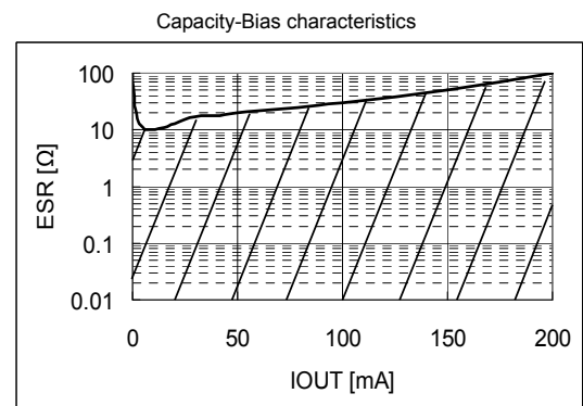
Stable area characteristics (Characteristics example)
