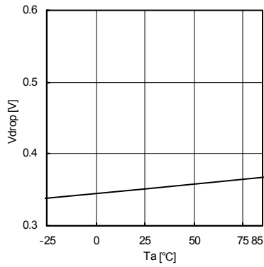
Fig.16 Minimum dropout Voltage 1 (Vcc=3.3V, Io=-0.5A)
