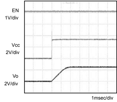
Fig.3 Input sequence 1 C_o=1\mu\text{F}
