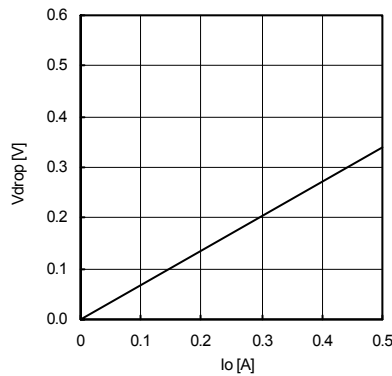
Fig.20 Minimum dropout Voltage 2 (Vcc=2.4V, Ta=25°C)
