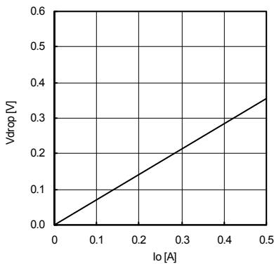
Fig.22 Minimum dropout Voltage 4 (Vcc=5.0V, Ta=25°C)
