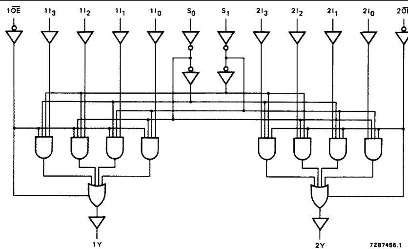
Fig.5 Logic diagram.
