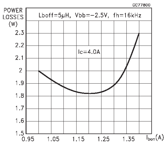
Power Losses At 16 KHz
