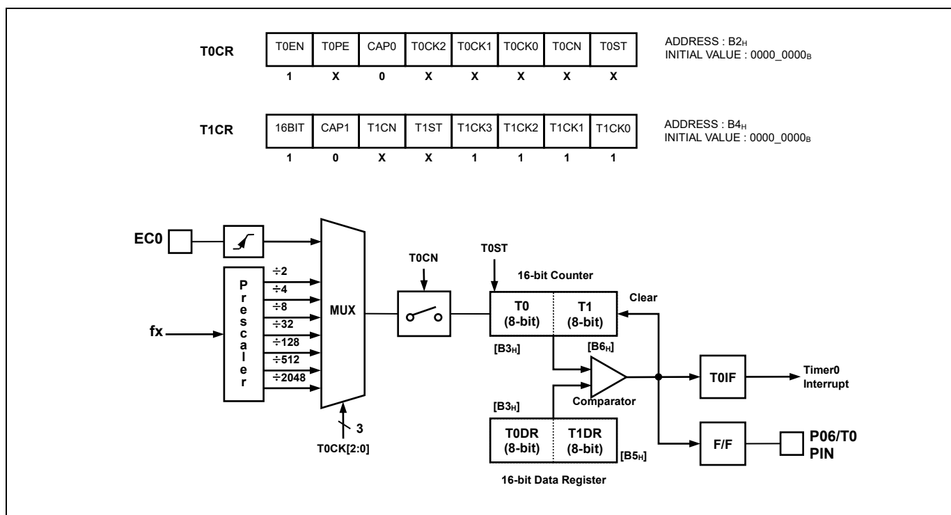
Figure 11.9 16-bit Timer/Counter for Time 0, 1
