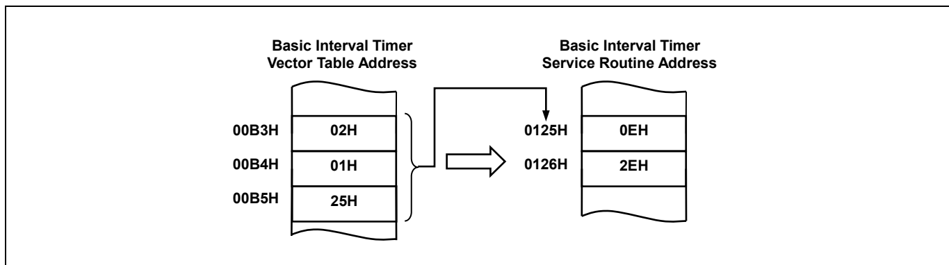
Figure 10.7 Correspondence between Vector Table Address and the Entry Address of ISR
