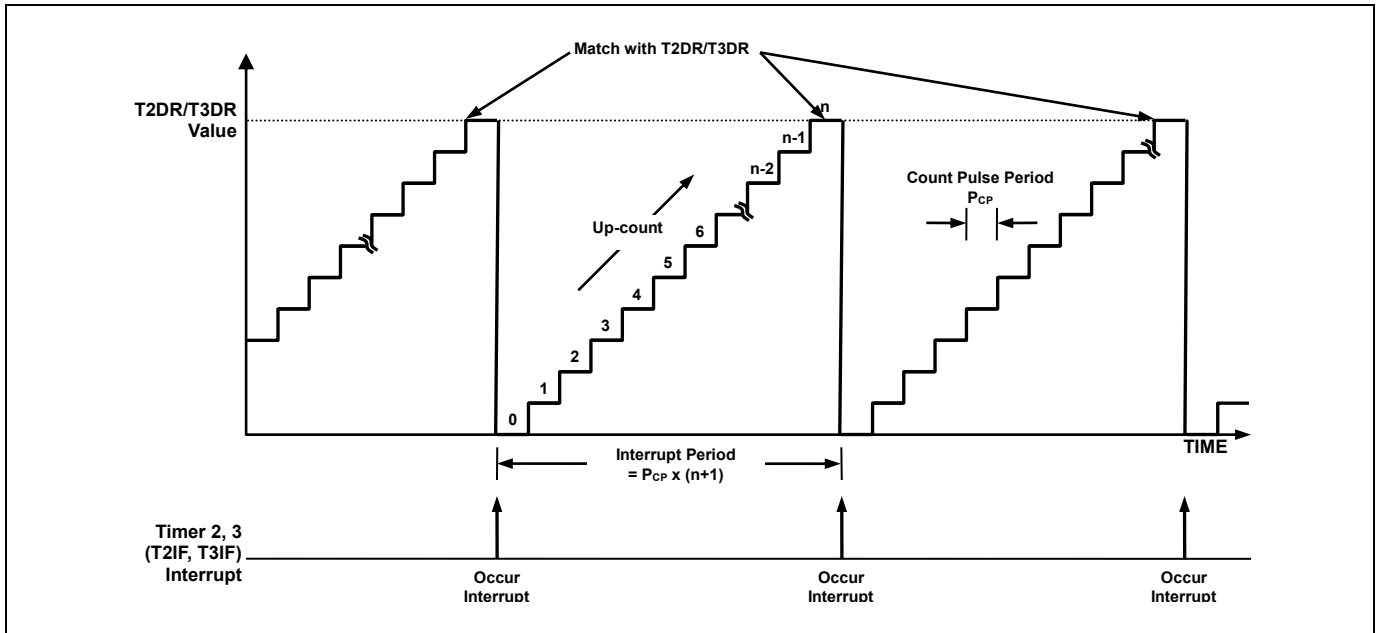
Figure 11.27 Timer/Event Counter 2, 3 Example
