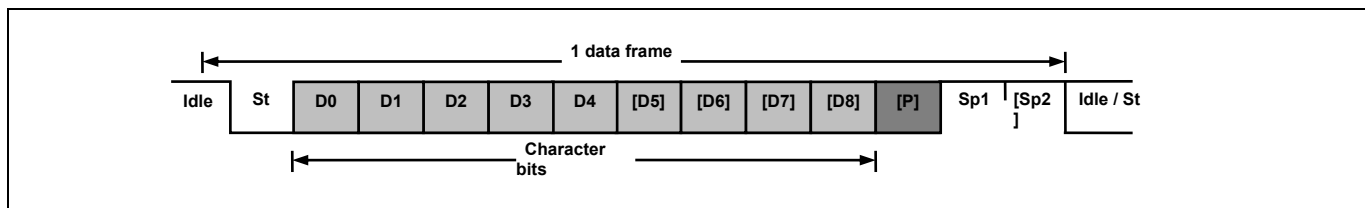
Figure 11.42 frame format
