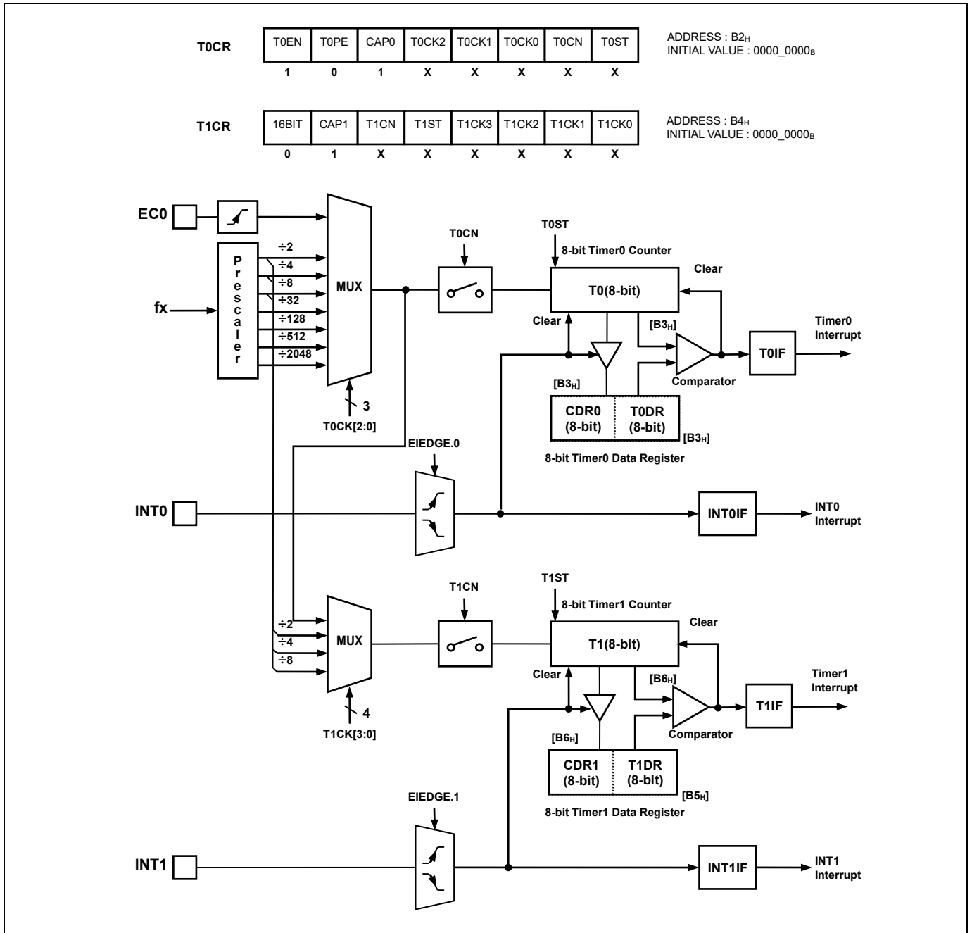
Figure 11.10 8-bit Capture Mode for Timer 0, 1
