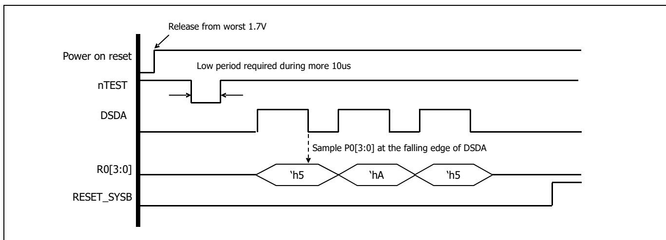
Figure 15.11 Byte-parallel mode
