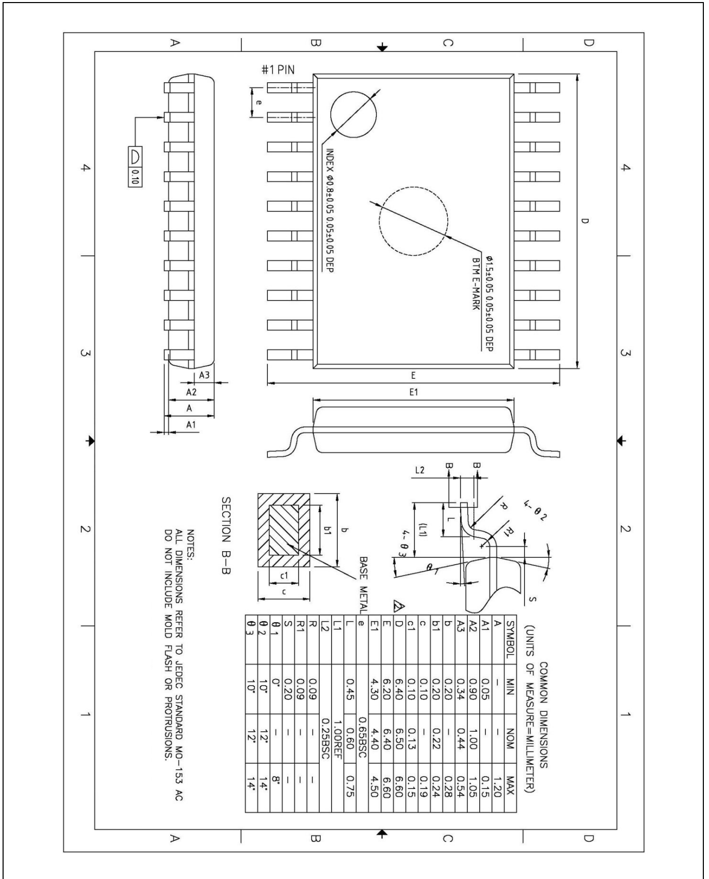
Figure 4.9 20-Pin TSSOP Package
