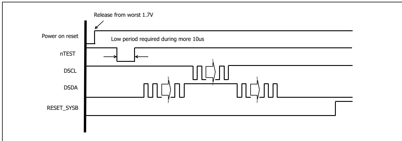
Figure 15.10 ISP mode
