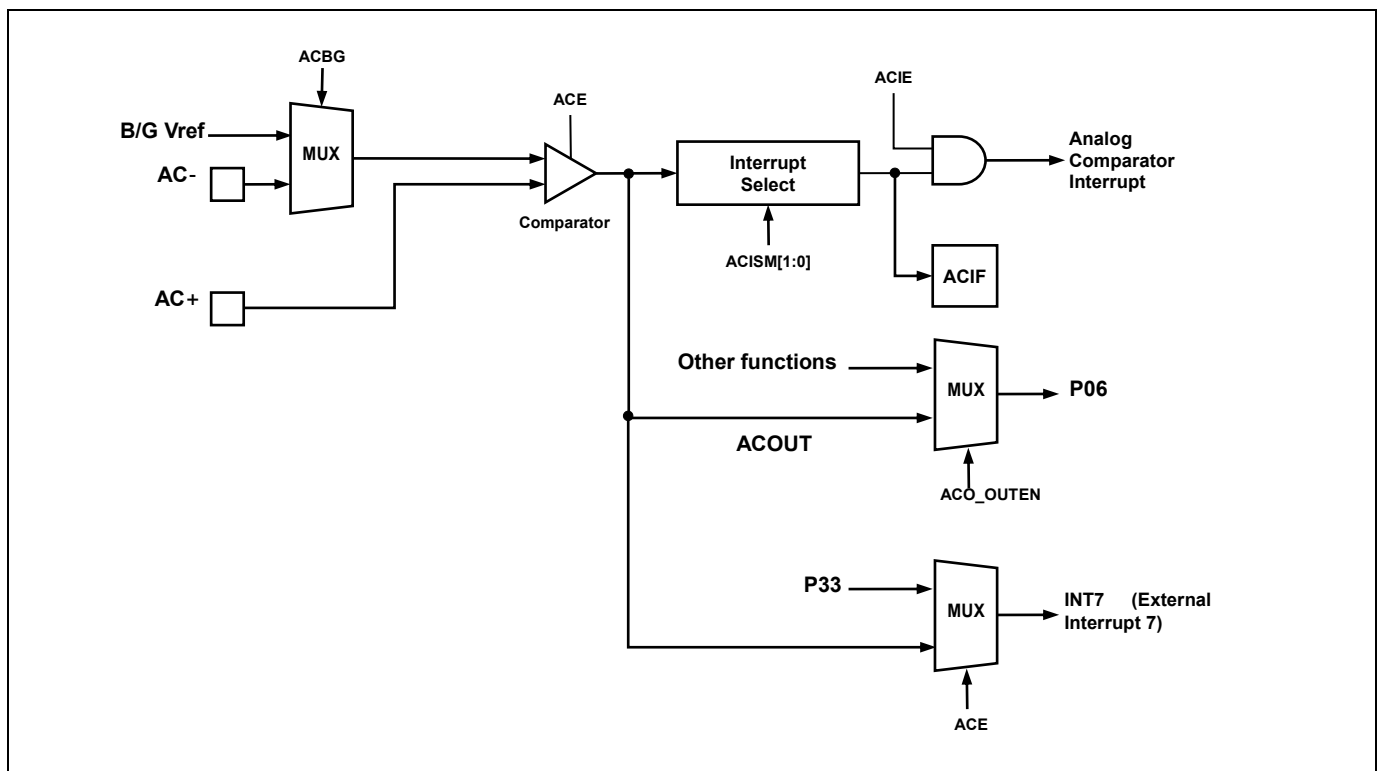
Figure 11.63 Analog Comparator Block Diagram
