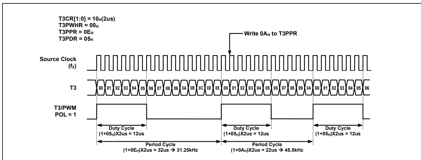
Figure 11.36 Example of Changing the Period in Absolute Duty Cycle at 4MHz
