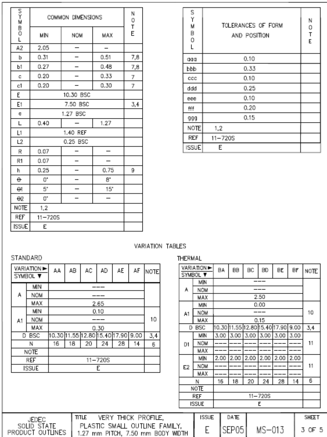
Figure 4.6 28-Pin SOP Package
