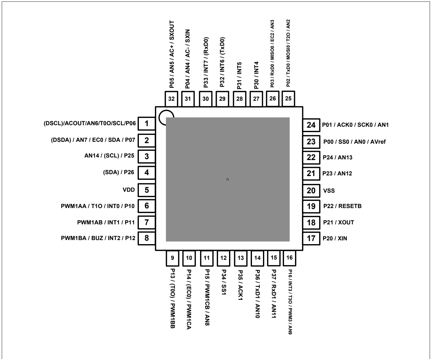
Figure 3.2 MC95FG308 32QFN pin assignment
