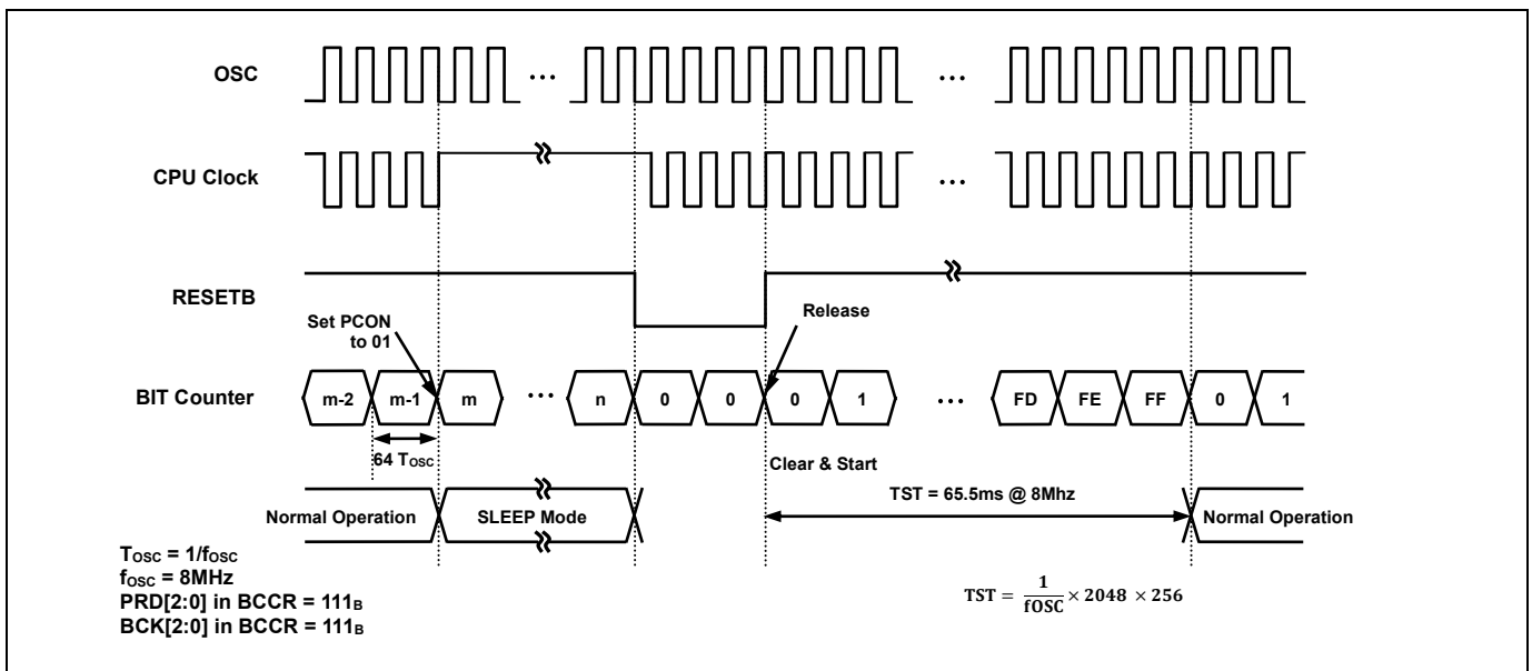
Figure 12.2 Figure 1 IDLE Mode Release Timing by /RESET
