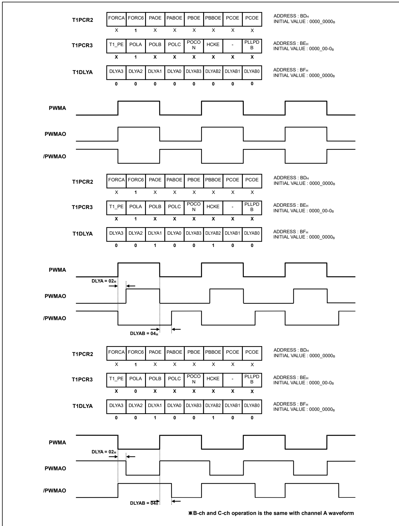
Figure 11.25 Example of PWM Delay
