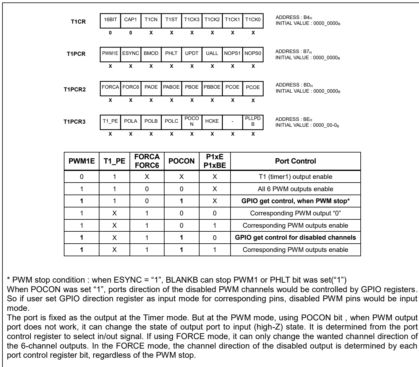
Figure 11.24 PWM Port control
