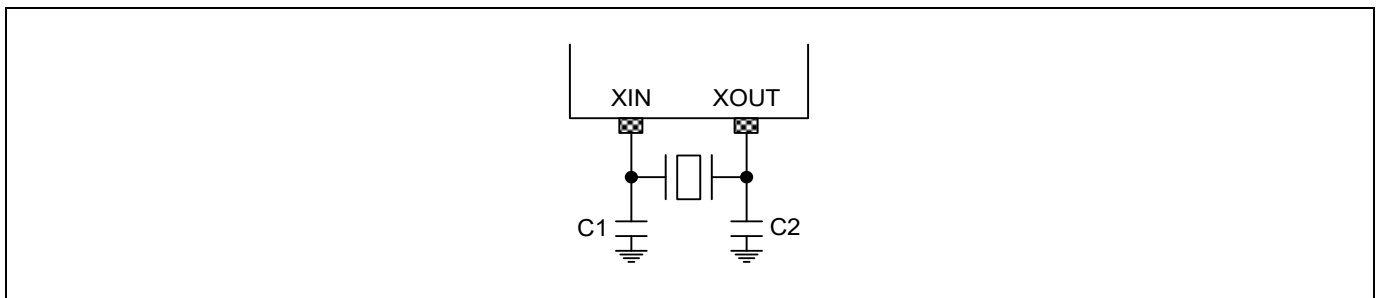
Figure 7.3 Crystal Oscillator
