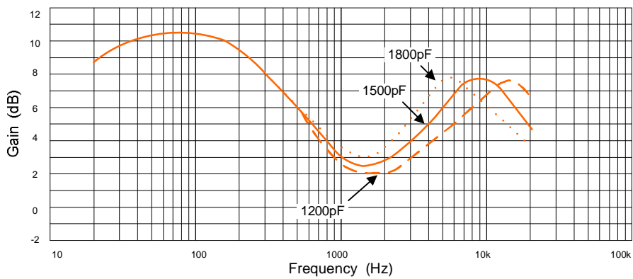
Fig.6 TL-OUTL Capacitors vs. Frequency Response
